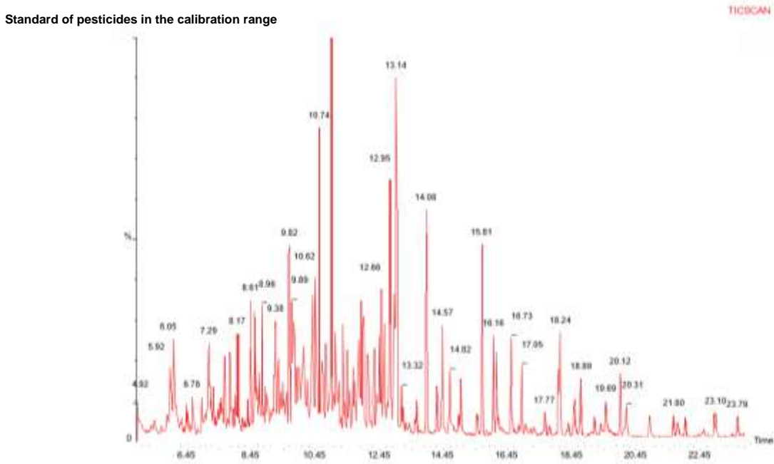
Fig 1: Chromatogram of the standard
