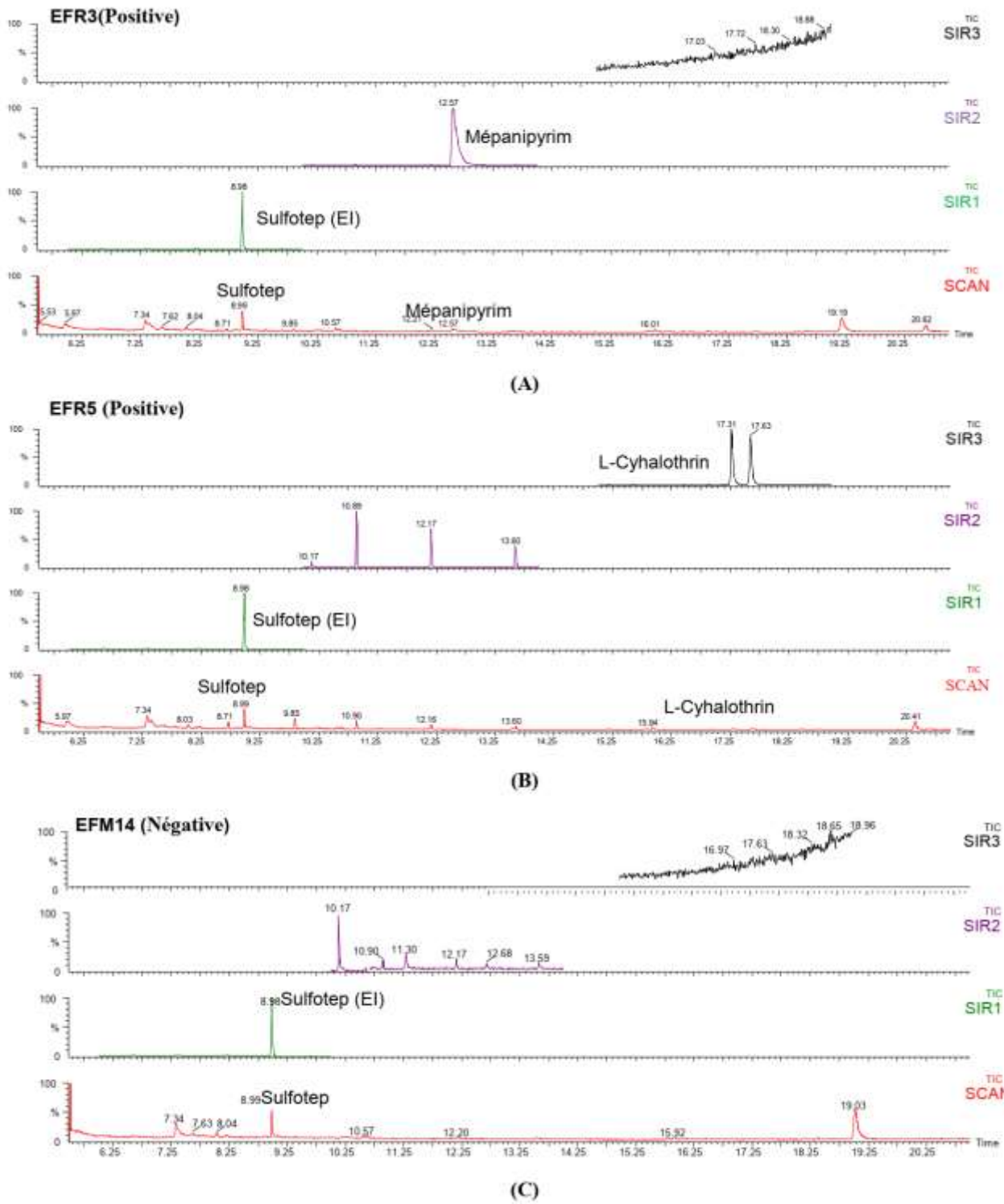
Fig 3 : Chromatograms of the samples (A, EFR3, B, EFR5 and C, EFM14)
